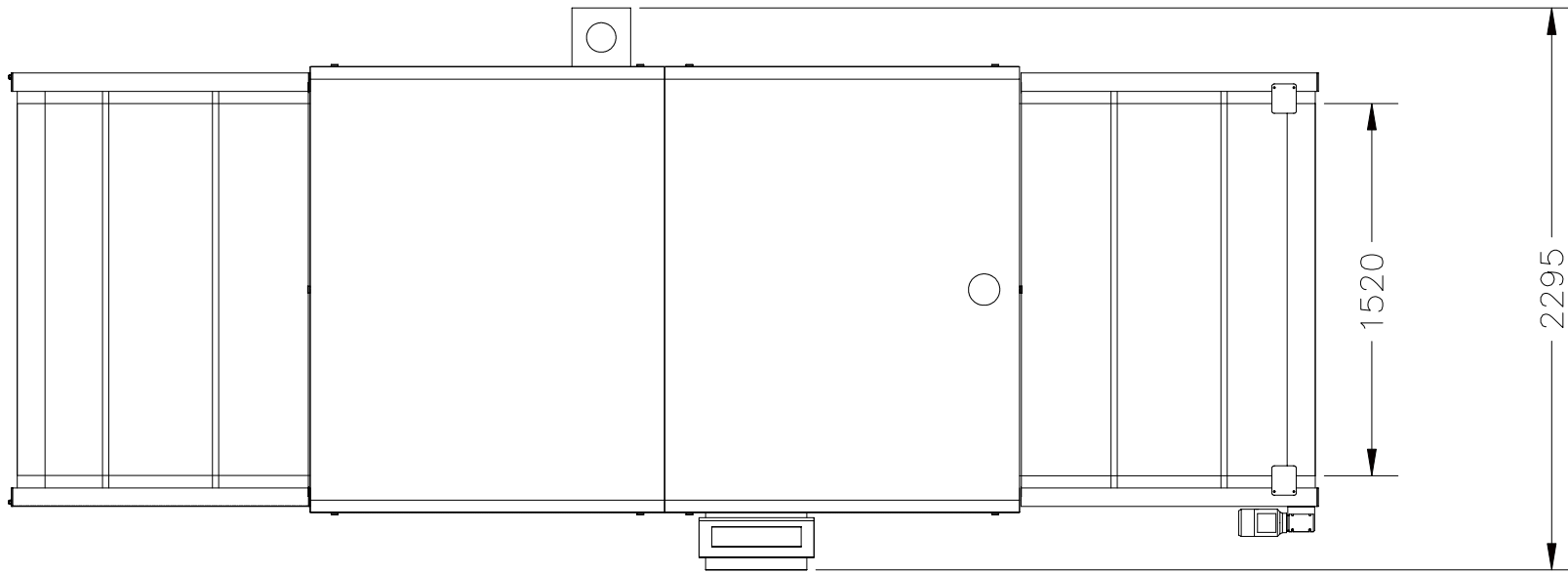
GAS / DIESEL DRYING TUNNEL GAL-60115 main view
