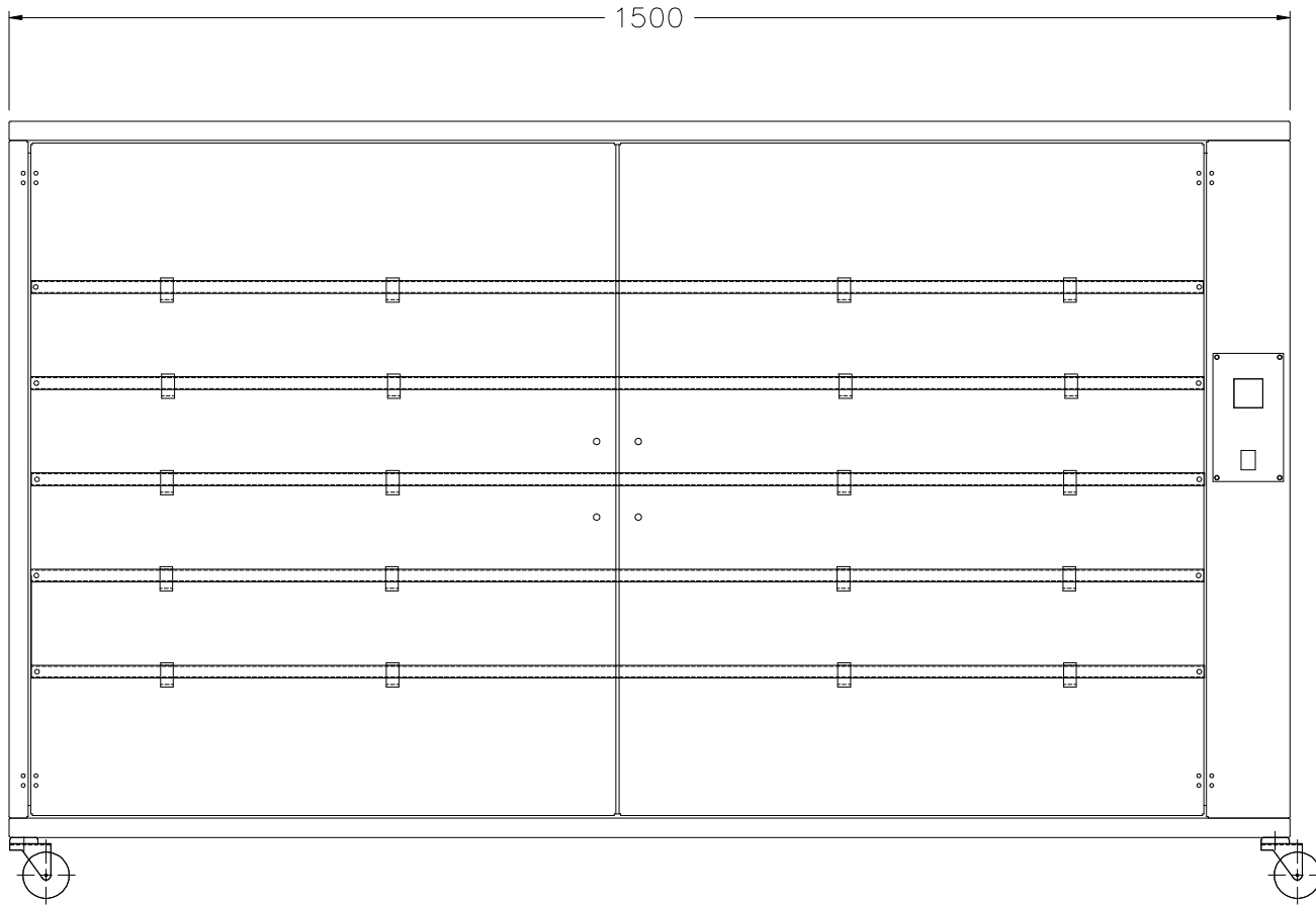
SED 120x90 MAIN VIEW
